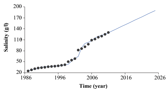
Fig.6 Water salinity plot of the Small Aral Sea
