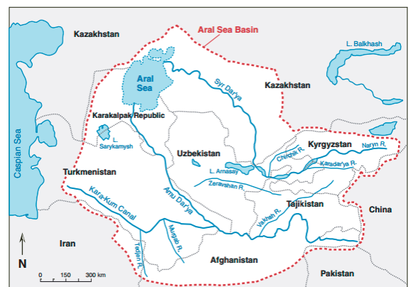
Fig.1 Aral Sea Basin (Micklin, 2007)
